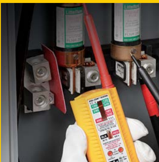
5-600V AC/DC Voltage Tester (61-076) Split-Jaw™ Smart Meter (61-096)
